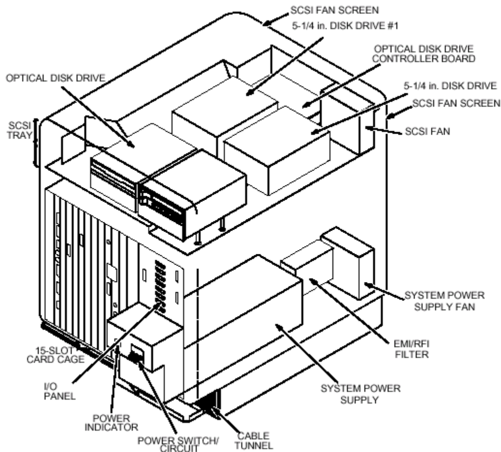
INSPECTION OF GENESIS COMPUTER FANS (COVERS REMOVED)
